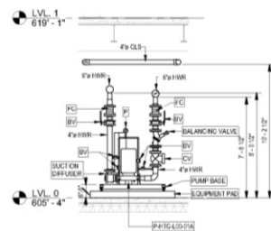
A SECTION MB.00E 1/4" = 1'-0"
