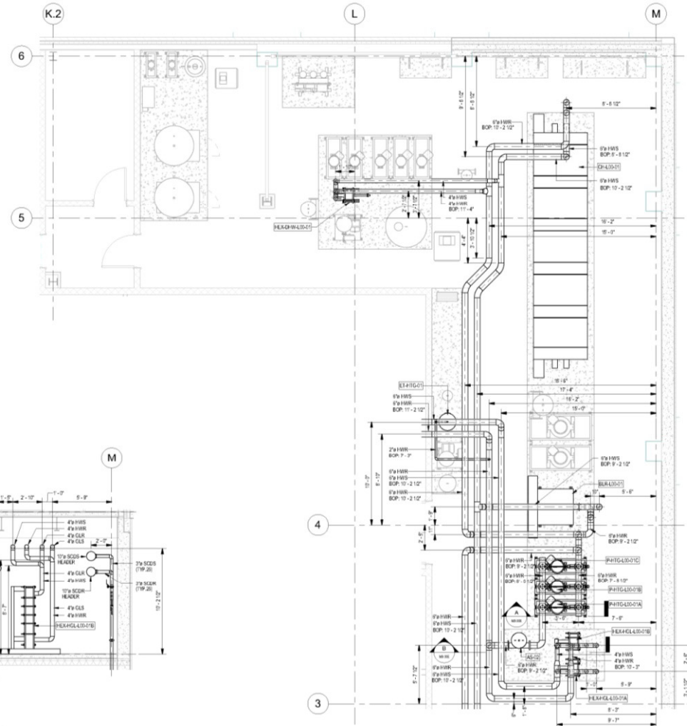
1 ENLARGE FLOOR PLAN MB.00E 1/4" = 1'-0"
