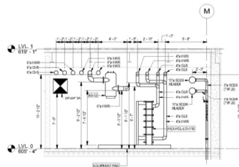
B SECTION MB.00E 1/4" = 1'-0"
