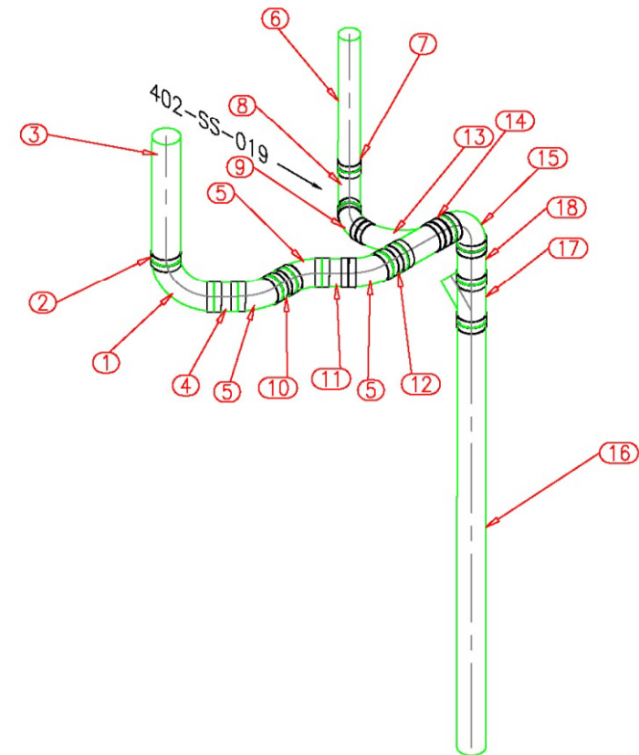
ISOMETRIC VIEW
