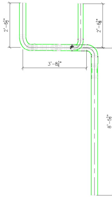
FRONT VIEW SCALE : 1/2" = 1'-0"
