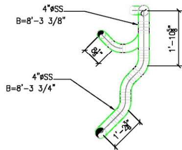
PLAN VIEW SCALE : 1/2" = 1'-0"
