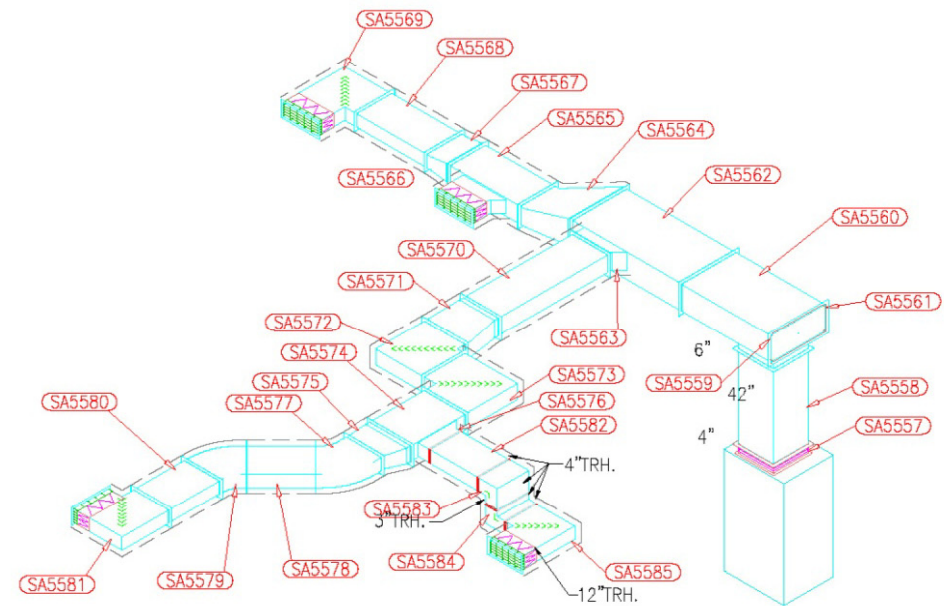
ISOMETRIC VIEW
