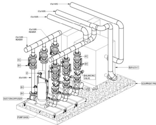
2 ISOMETRIC MB.00E
